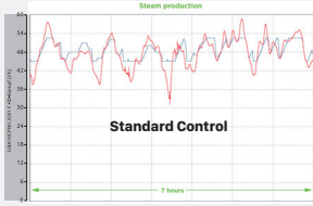
Steam production controlled by Standard Control
